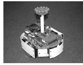
Figure 12: Linuxbot
