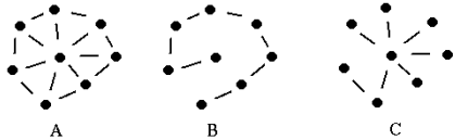
Figure 6: A graph(A) & two disjoint spanning trees(B,C)
