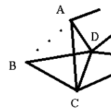
Figure 3: Shared neighbour
